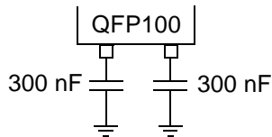
Figure 9. Recommended Connections for V_{REG}
