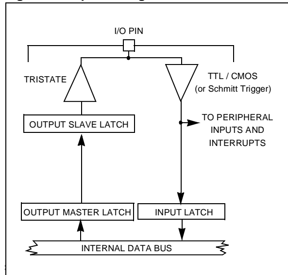
Figure 64. Input Configuration
