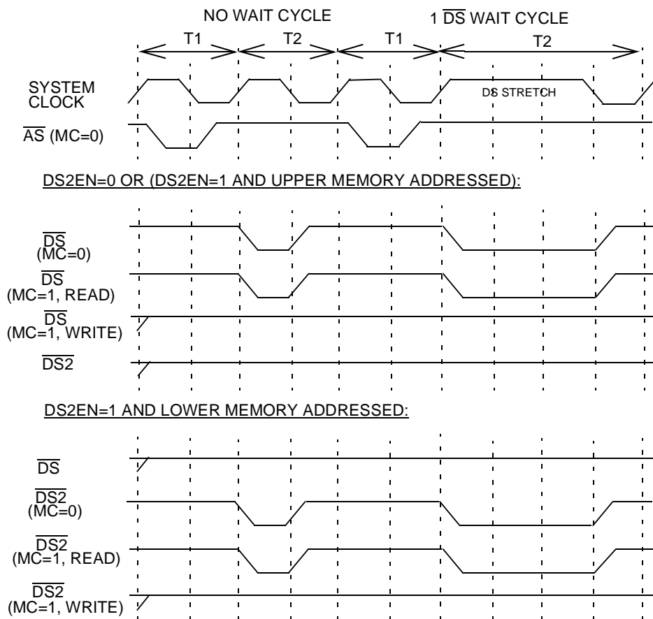
Figure 57. Effects of DS2EN on the behavior of \overline{DS} and \overline{DS2}
