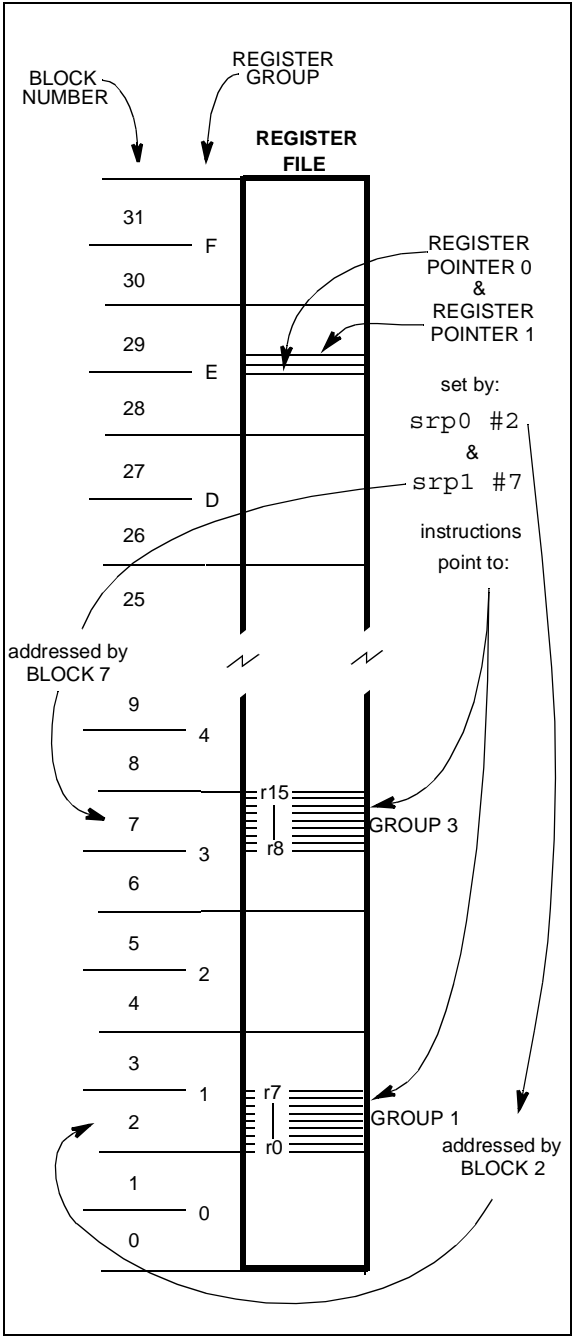
Figure 15. Pointing to two groups of 8 registers
