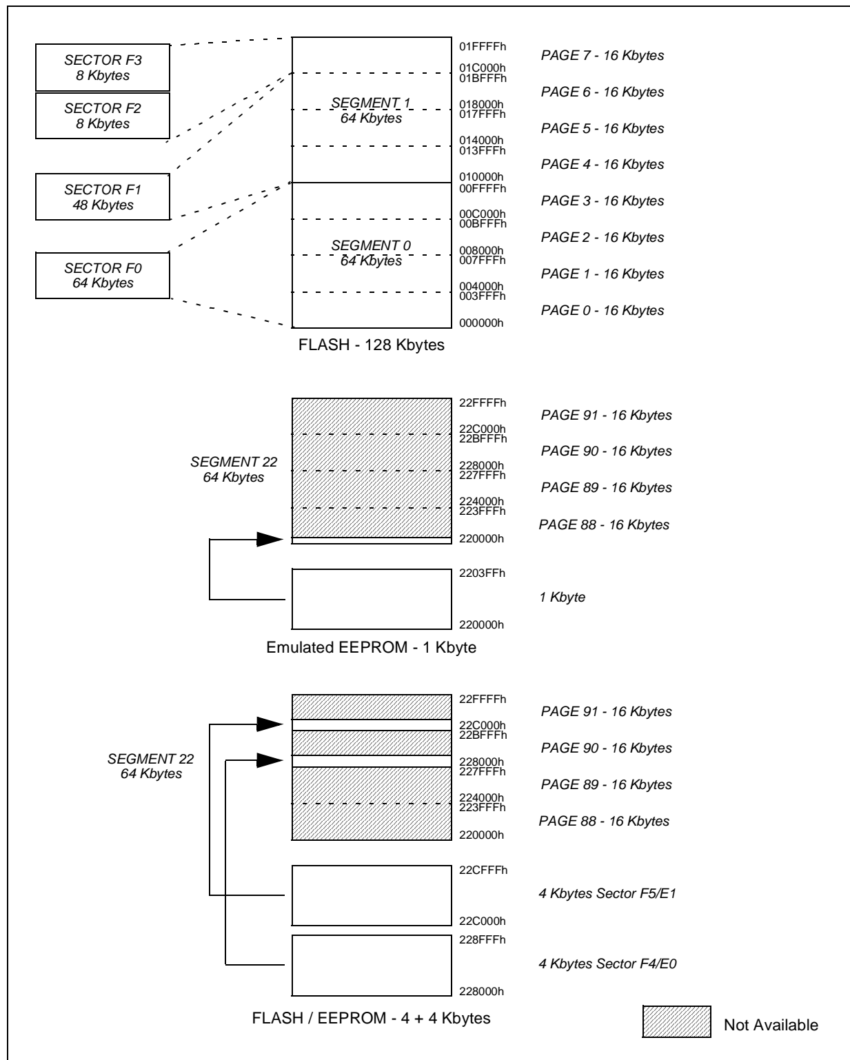
Figure 28. ST92F120JV1Q7/ST92F120V1Q7 User Memory Map (part 1)
