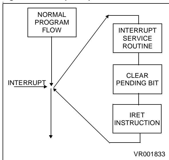
Figure 31. Interrupt Response
