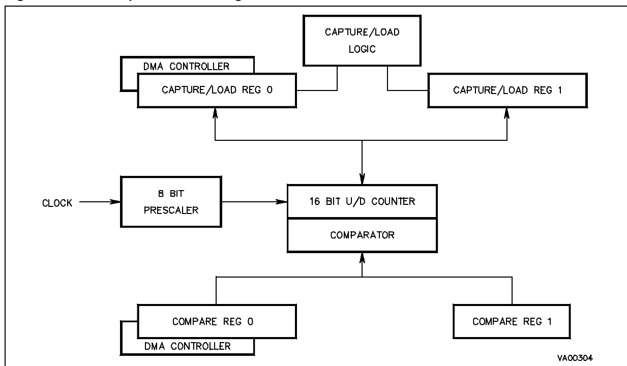
Figure 82. MFT Simplified Block Diagram
