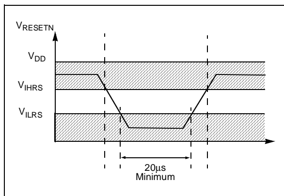
Figure 55. Recommended Signal to be Applied on Reset Pin
