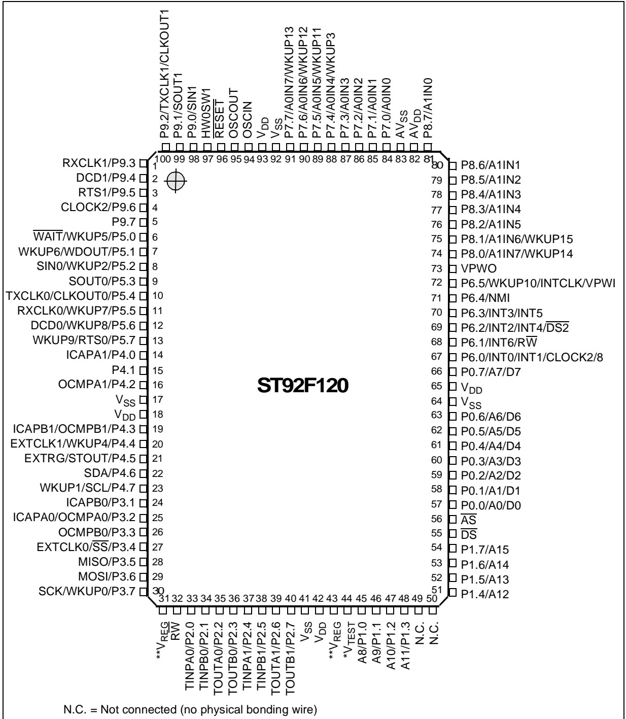
Figure 7. ST92F120: Pin Configuration (Top-view PQFP100)
