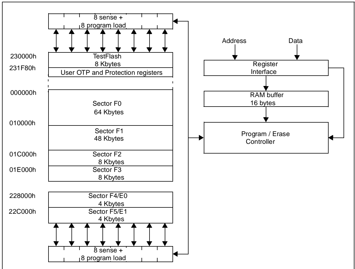
Figure 22. Flash Memory Structure (Example for 128K Flash device)
