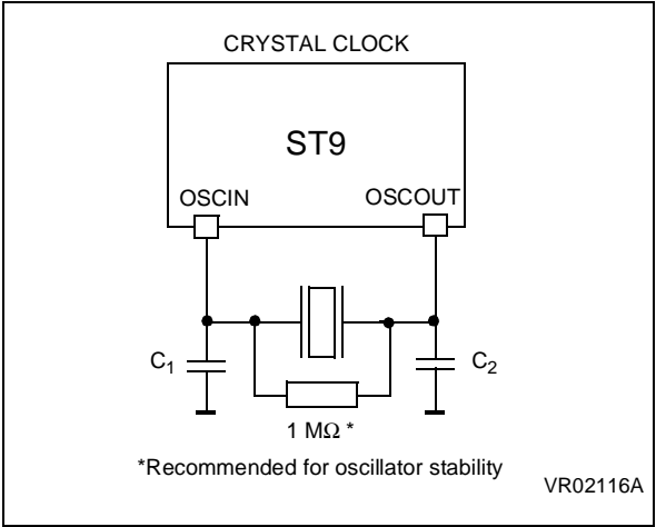
Figure 50. Crystal Oscillator
