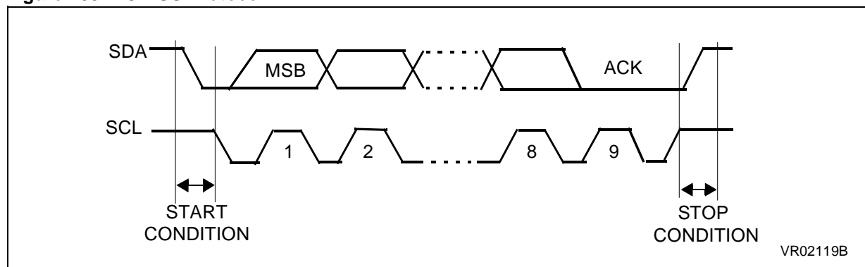
Figure 105. I 2 C BUS Protocol
