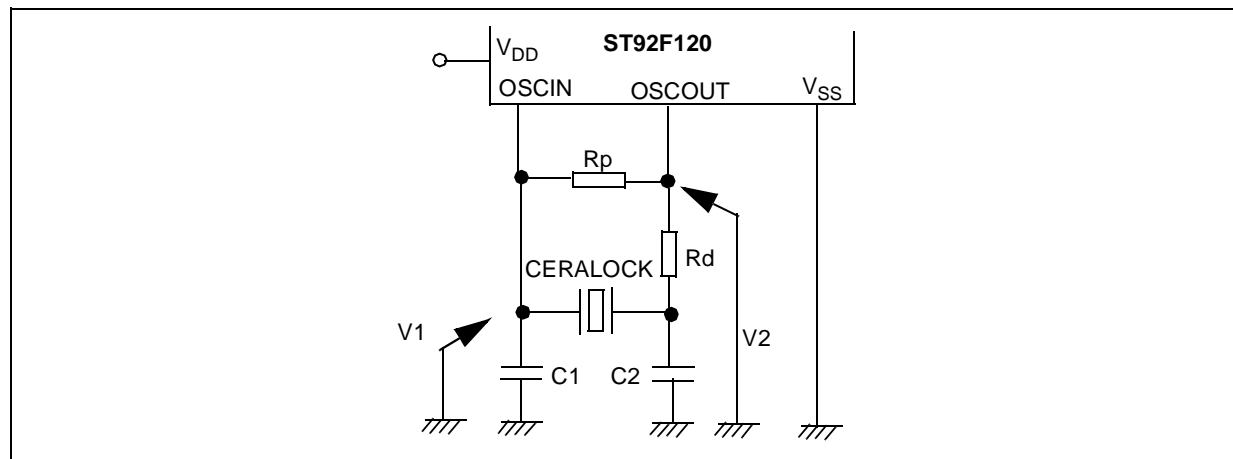
Figure 53. Test Circuit
