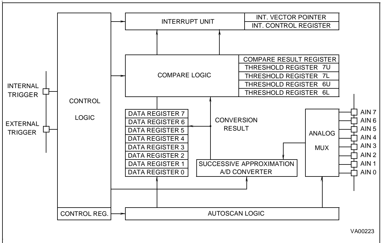
Figure 120. Block Diagram
