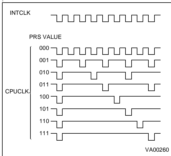
Figure 46. CPU Clock Prescaling
