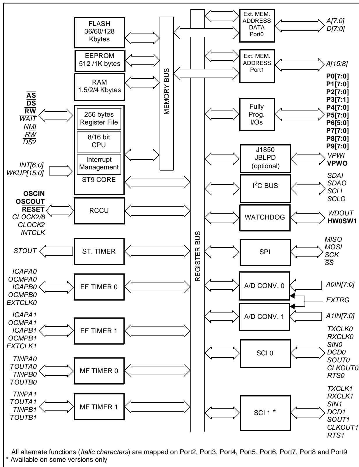
Figure 1. ST92F120JV: Architectural Block Diagram (PQFP100 version)
