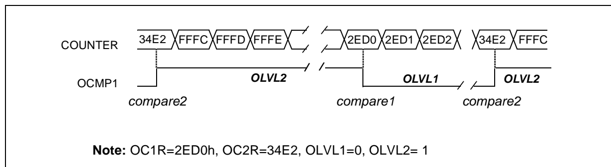
Figure 81. Pulse Width Modulation Mode Timing
