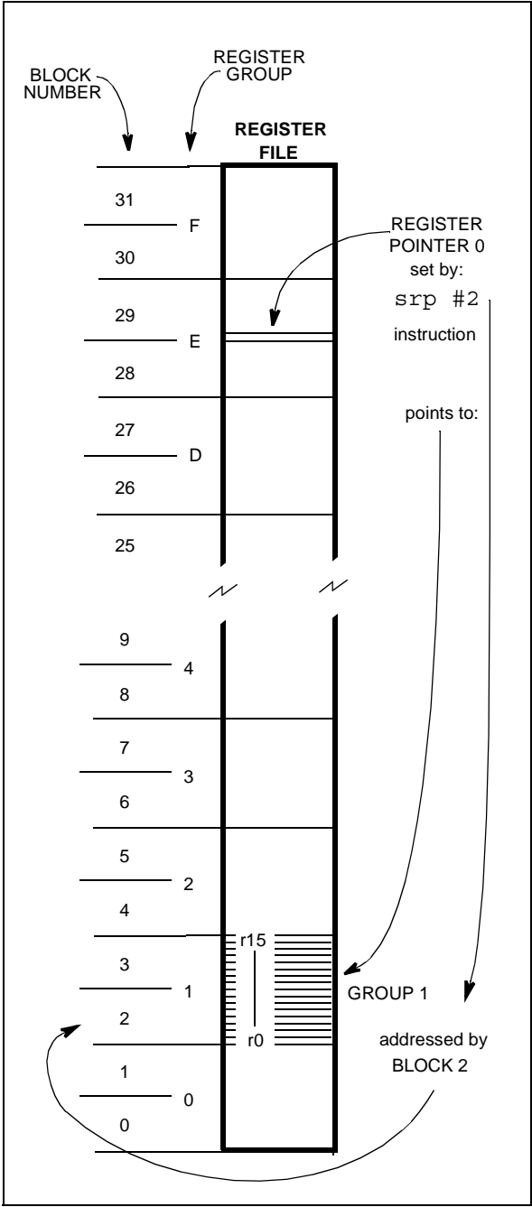
Figure 14. Pointing to a single group of 16 registers
