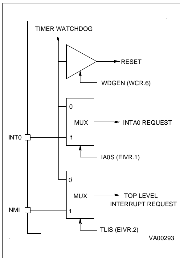
Figure 70. Interrupt Sources
