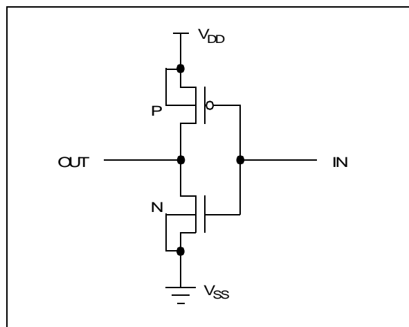
Figure 2. CMOS Basic Inverter
