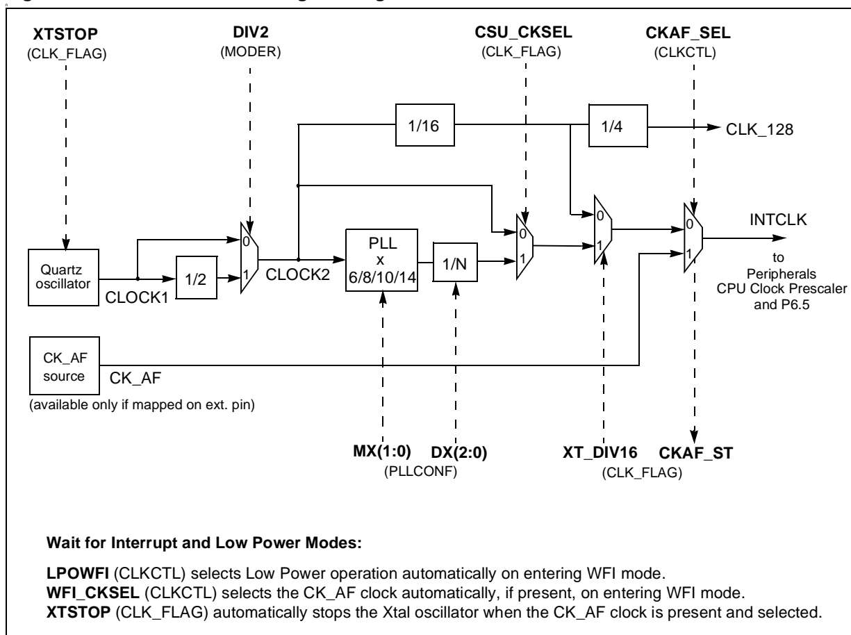
Figure 45. Clock Control Unit Programming
