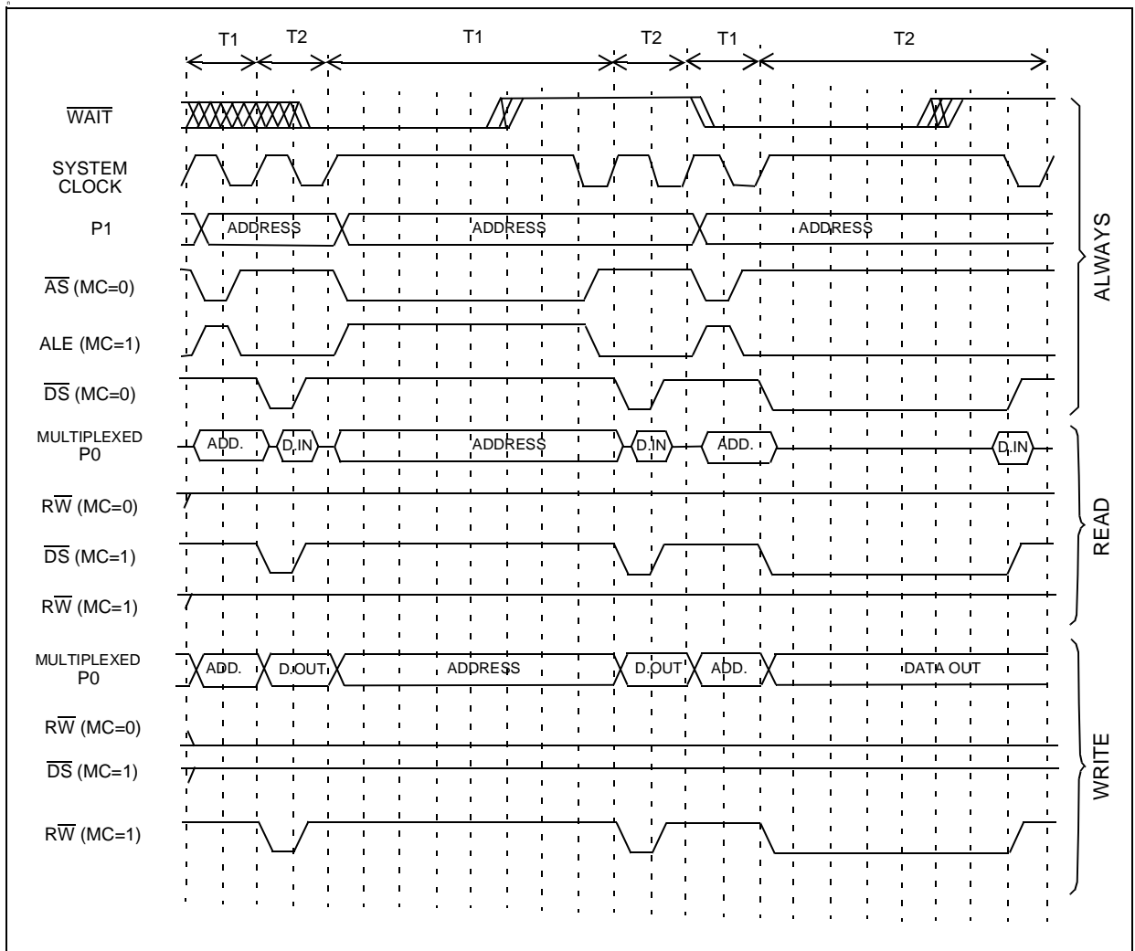
Figure 59. External Memory Read/Write Sequence with External Wait ( \overline{WAIT} pin)
