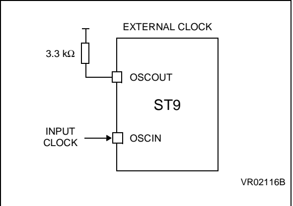
Figure 52. External Clock
