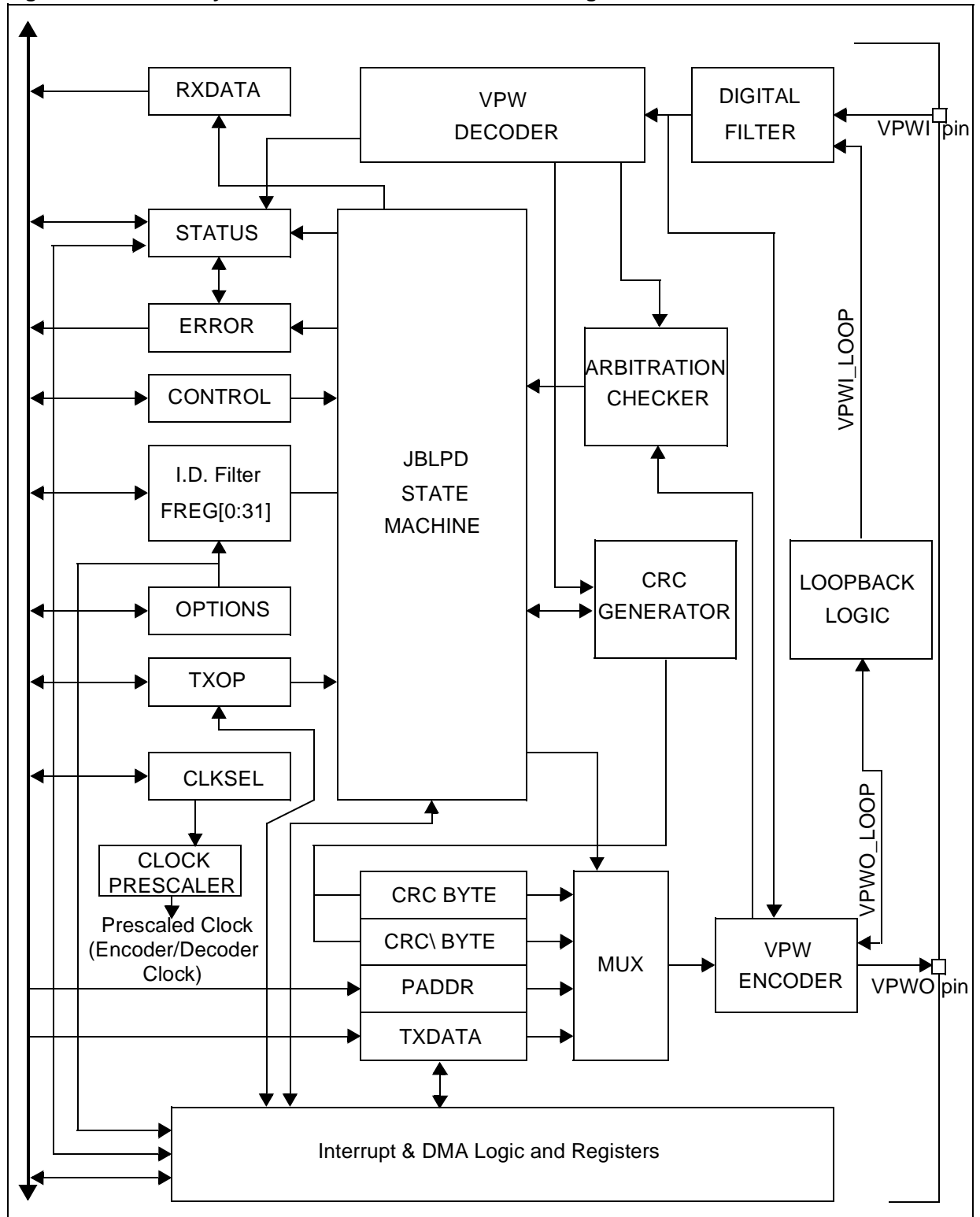
Figure 108. JBLPD Byte Level Protocol Decoder Block Diagram
