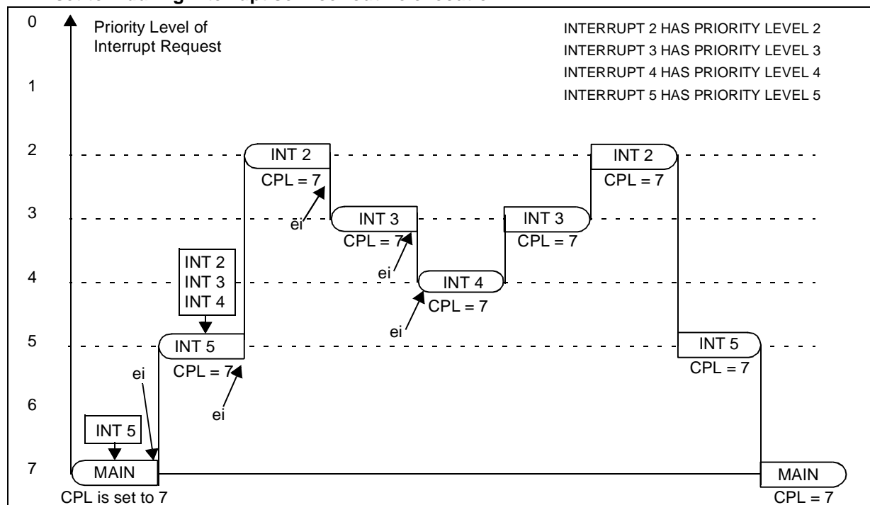
Figure 34. Complex Example of a Sequence of Interrupt Requests with:
