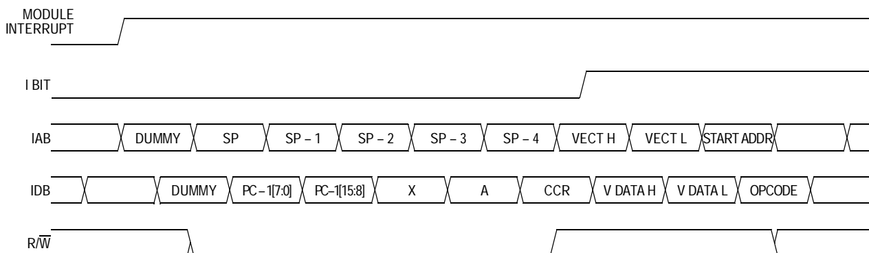
Figure 9-8. Interrupt Entry
