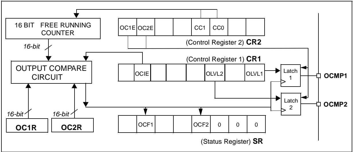
Figure 58. Output Compare Block Diagram
