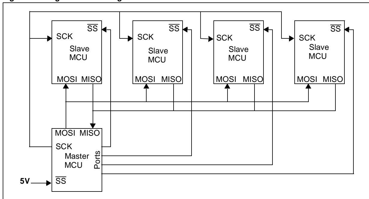
Figure 76. Single Master Configuration
