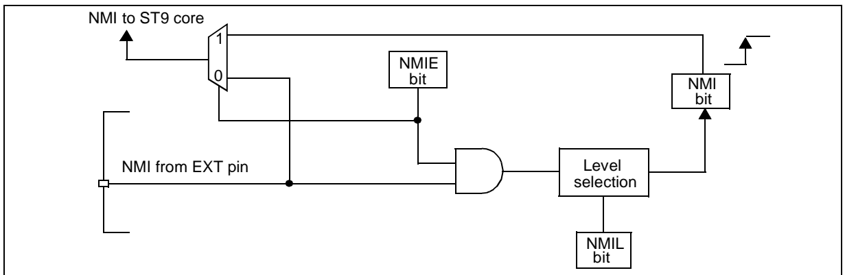
Figure 70. NMI management by the IMC peripheral
