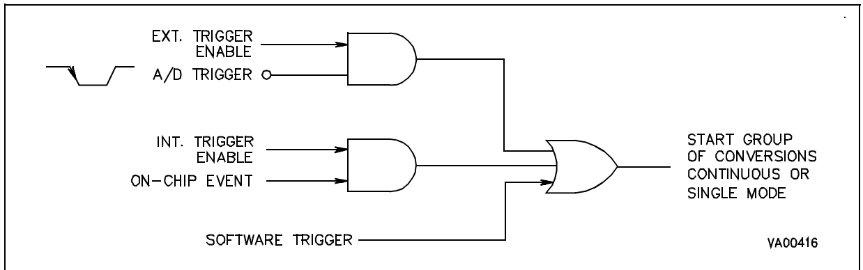
Figure 78. A/D Trigger Source
