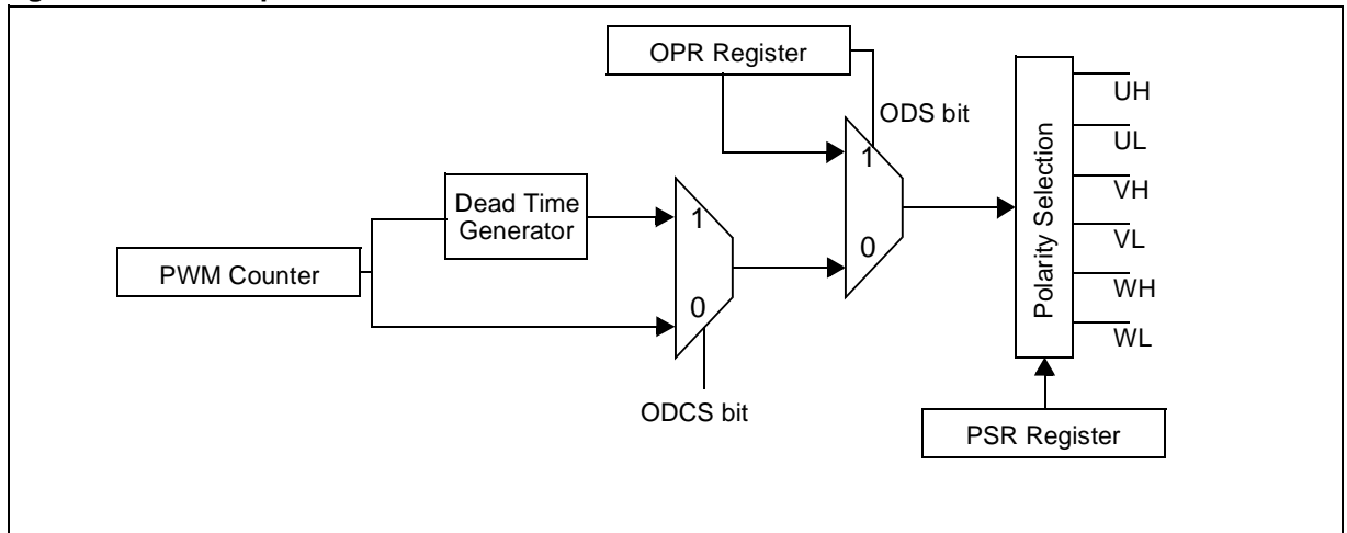
Figure 69. IMC Output selection.
