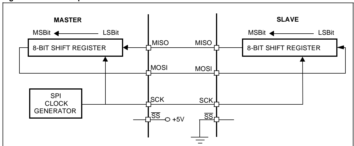
Figure 71. Serial Peripheral Interface Master/Slave
