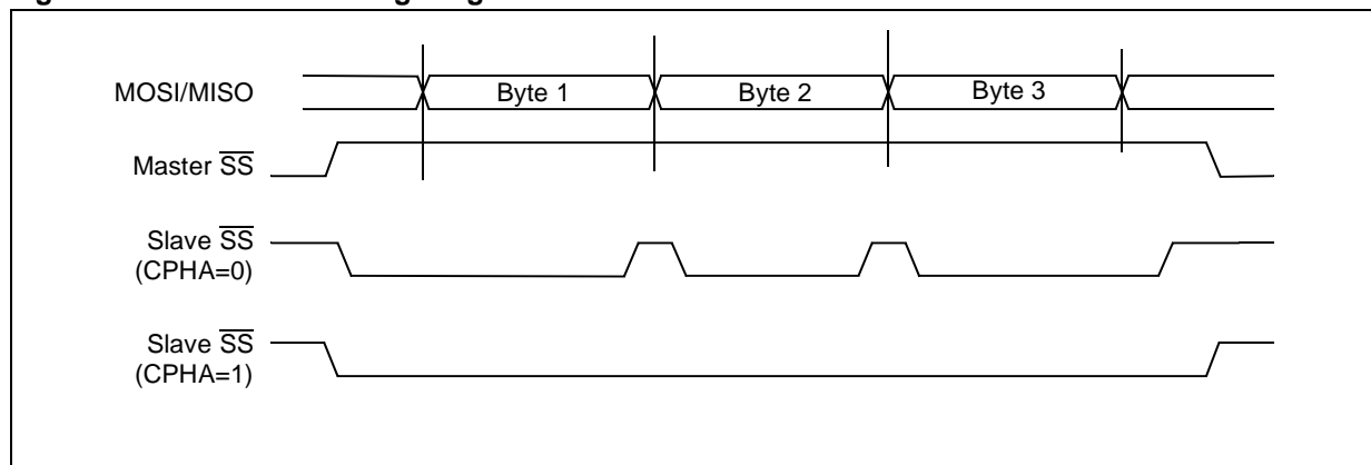
Figure 73. CPHA / \overline{SS} Timing Diagram
