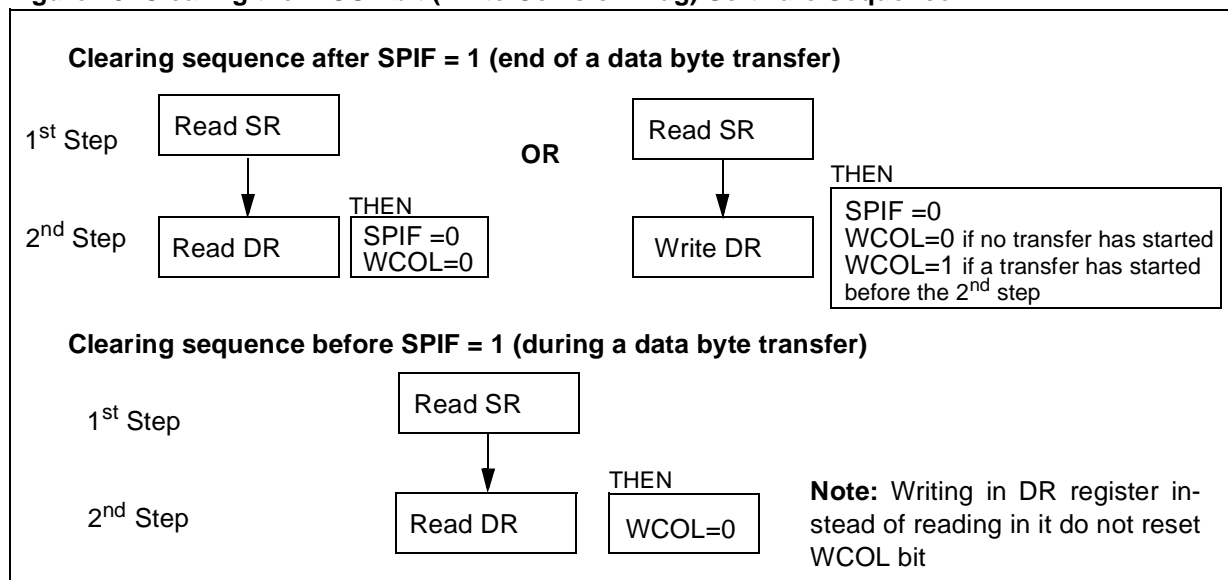
Figure 75. Clearing the WCOL bit (Write Collision Flag) Software Sequence
