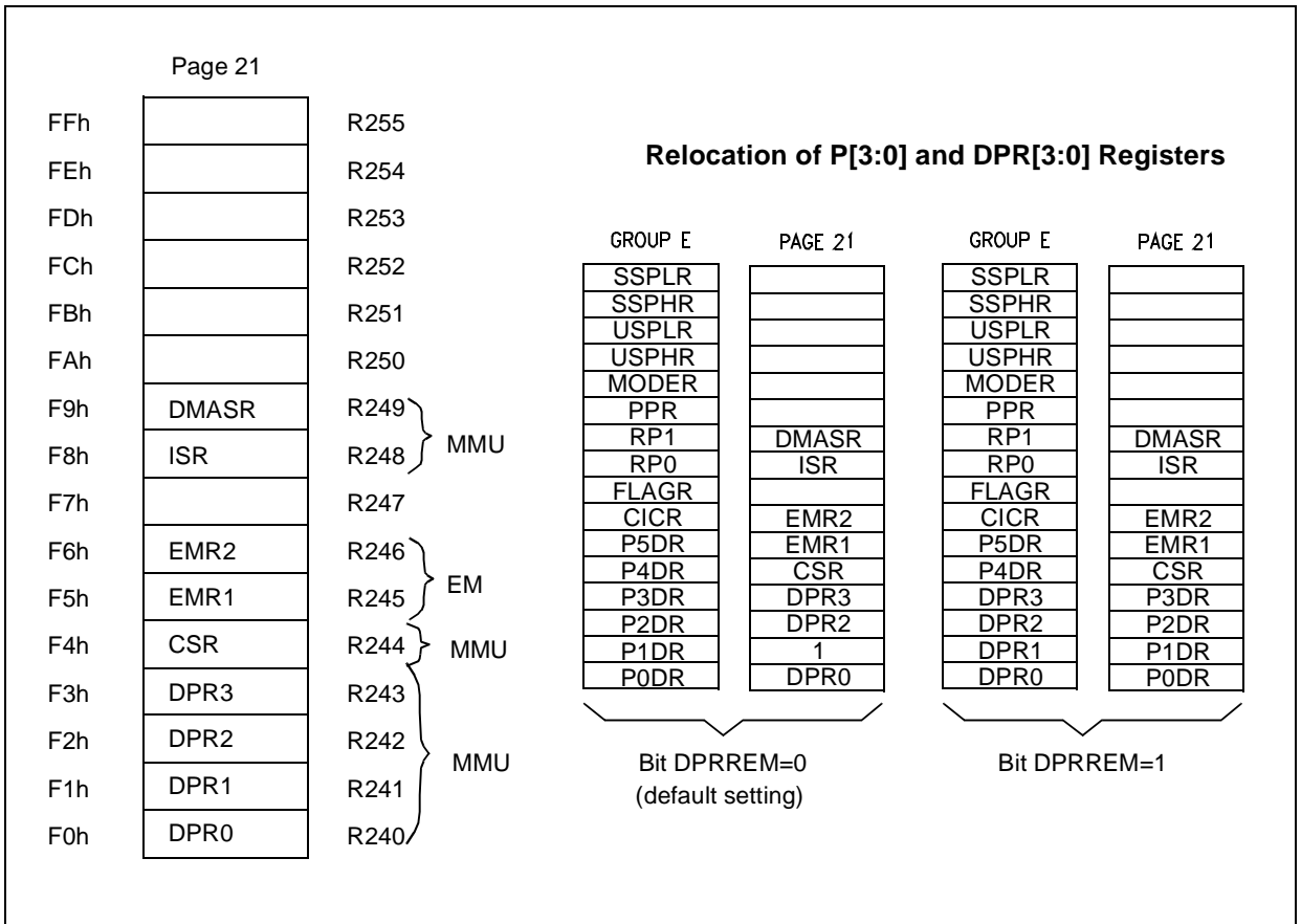
Figure 11. Page 21 Registers
