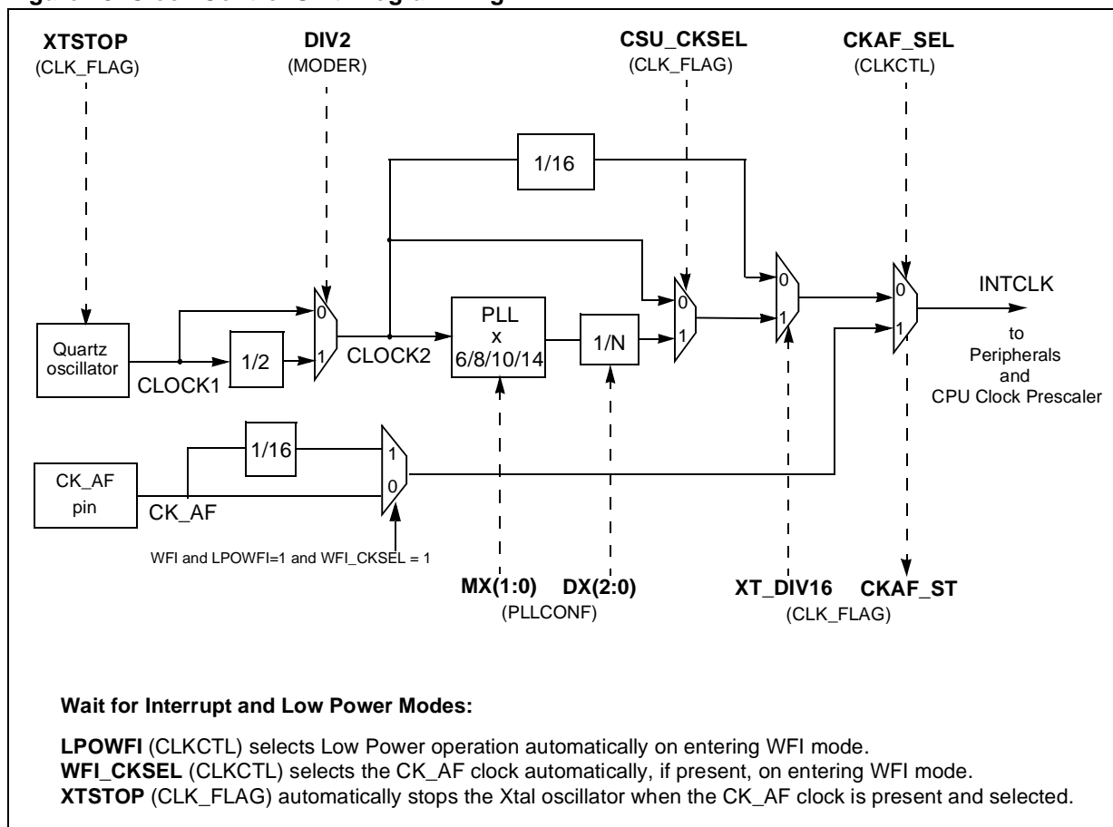
Figure 28. Clock Control Unit Programming
