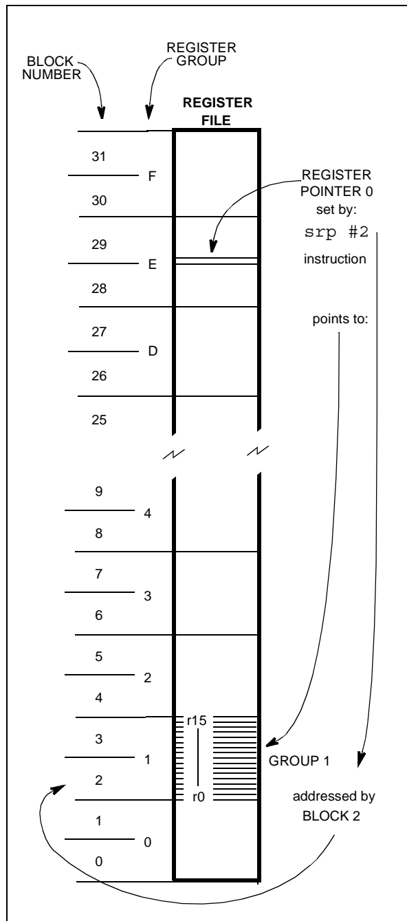
Figure 7. Pointing to a single group of 16 registers
