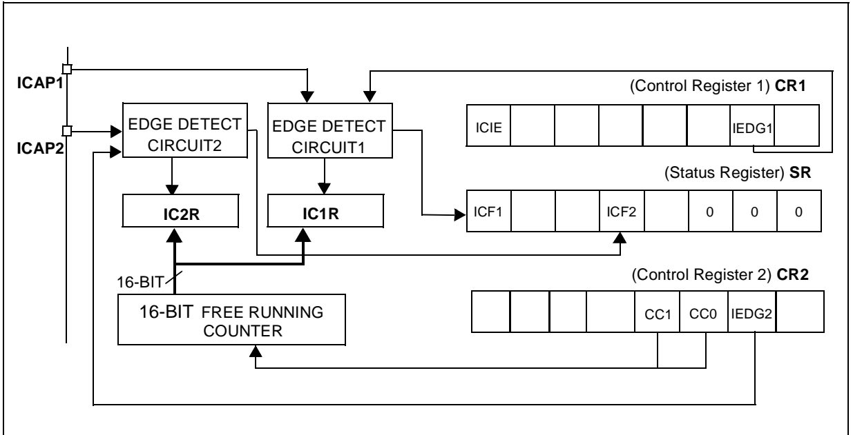
Figure 56. Input Capture Block Diagram
