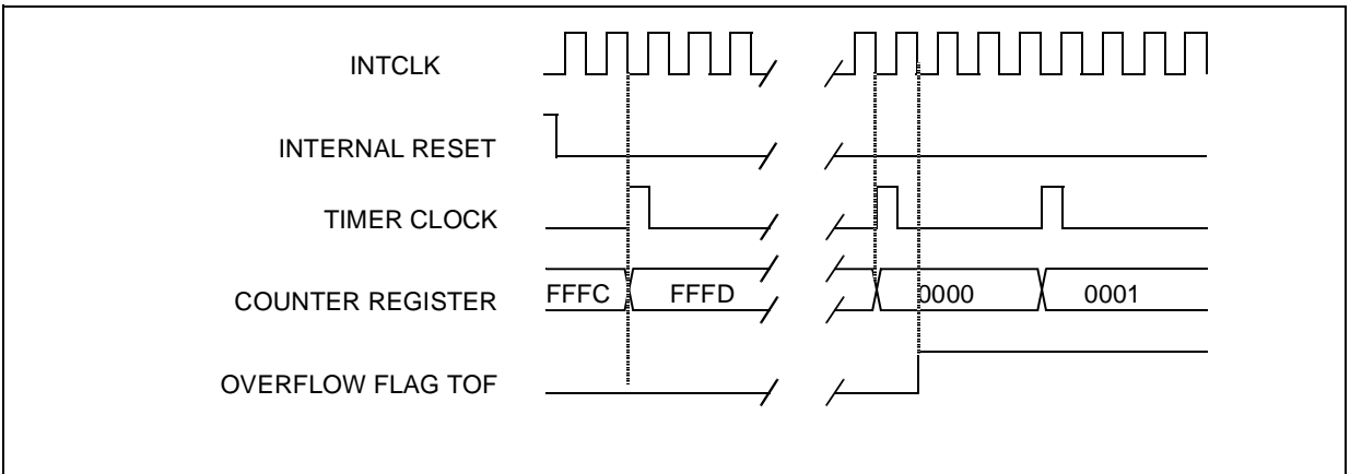
Figure 54. Counter Timing Diagram, INTCLK divided by 4
