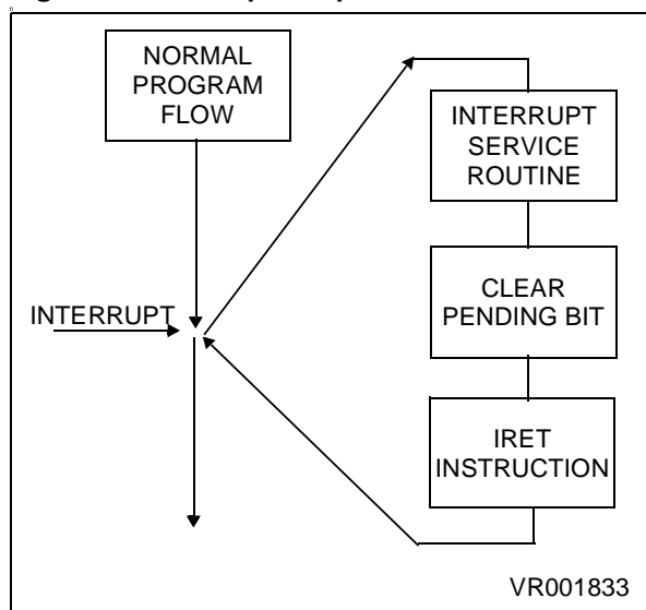
Figure 15. Interrupt Response
