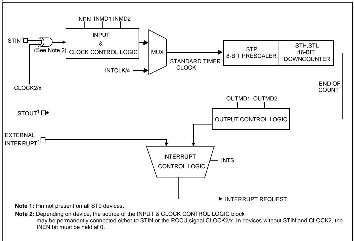
Figure 51. Standard Timer Block Diagram
