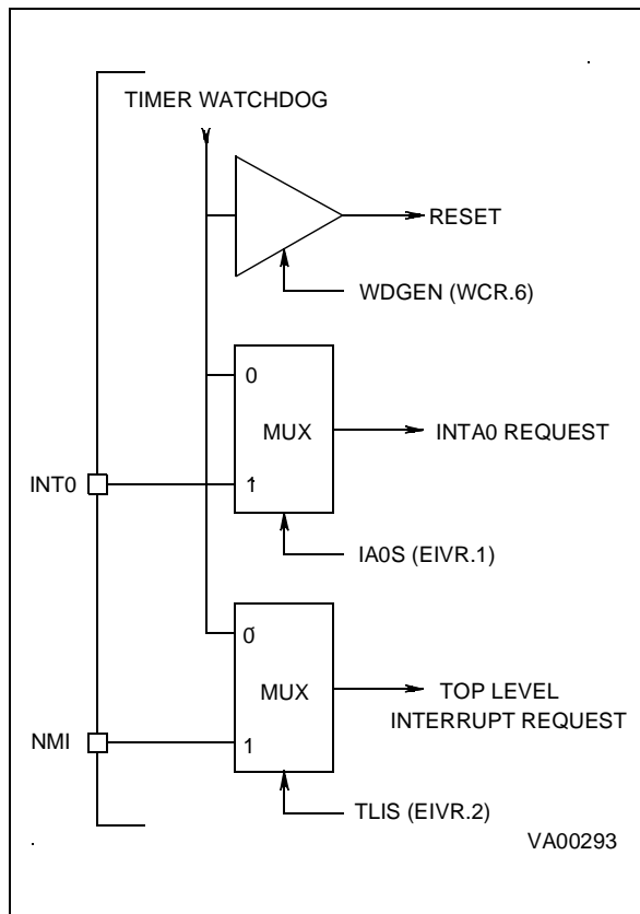
Figure 50. Interrupt Sources
