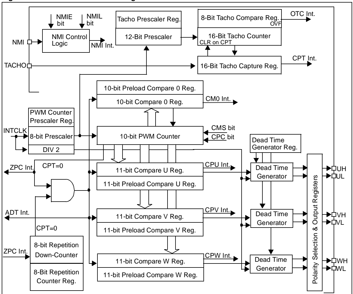
Figure 62. IMC Controller Block Diagram
