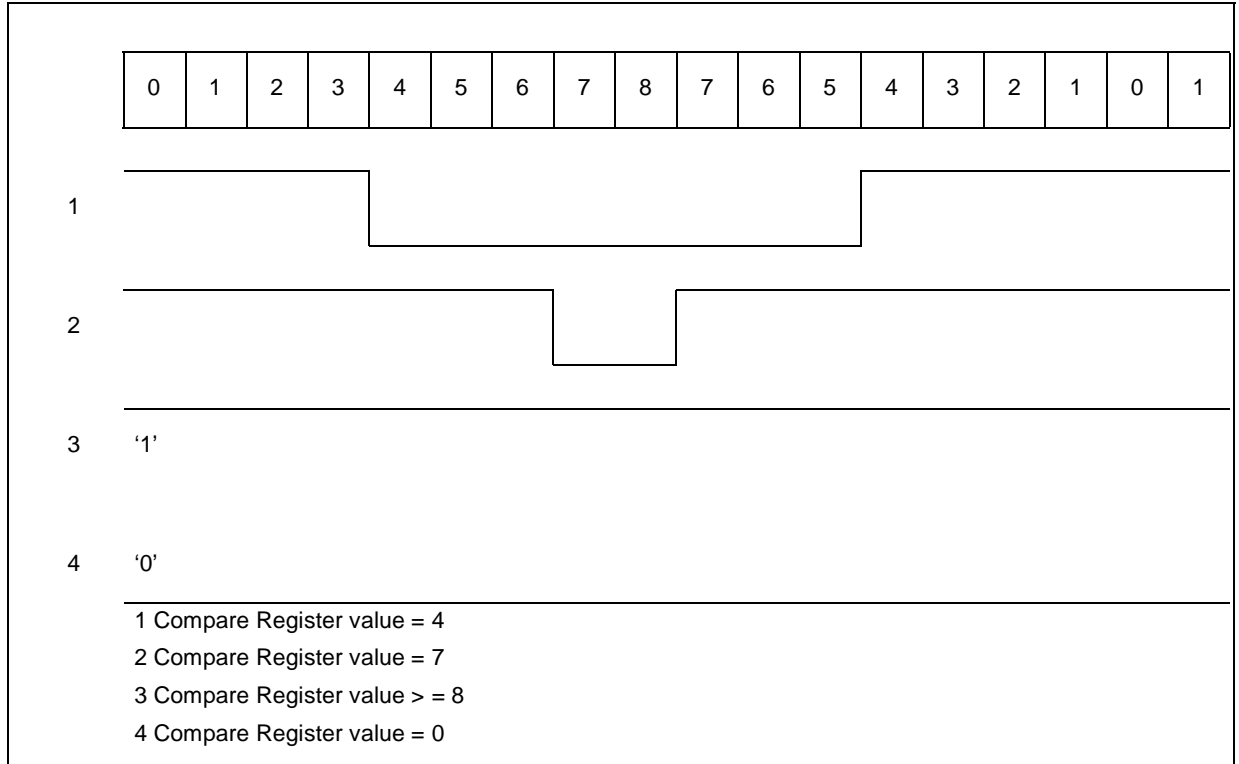
Figure 64. Zerocentered PWM Waveforms (Compare 0 Register = 8)
