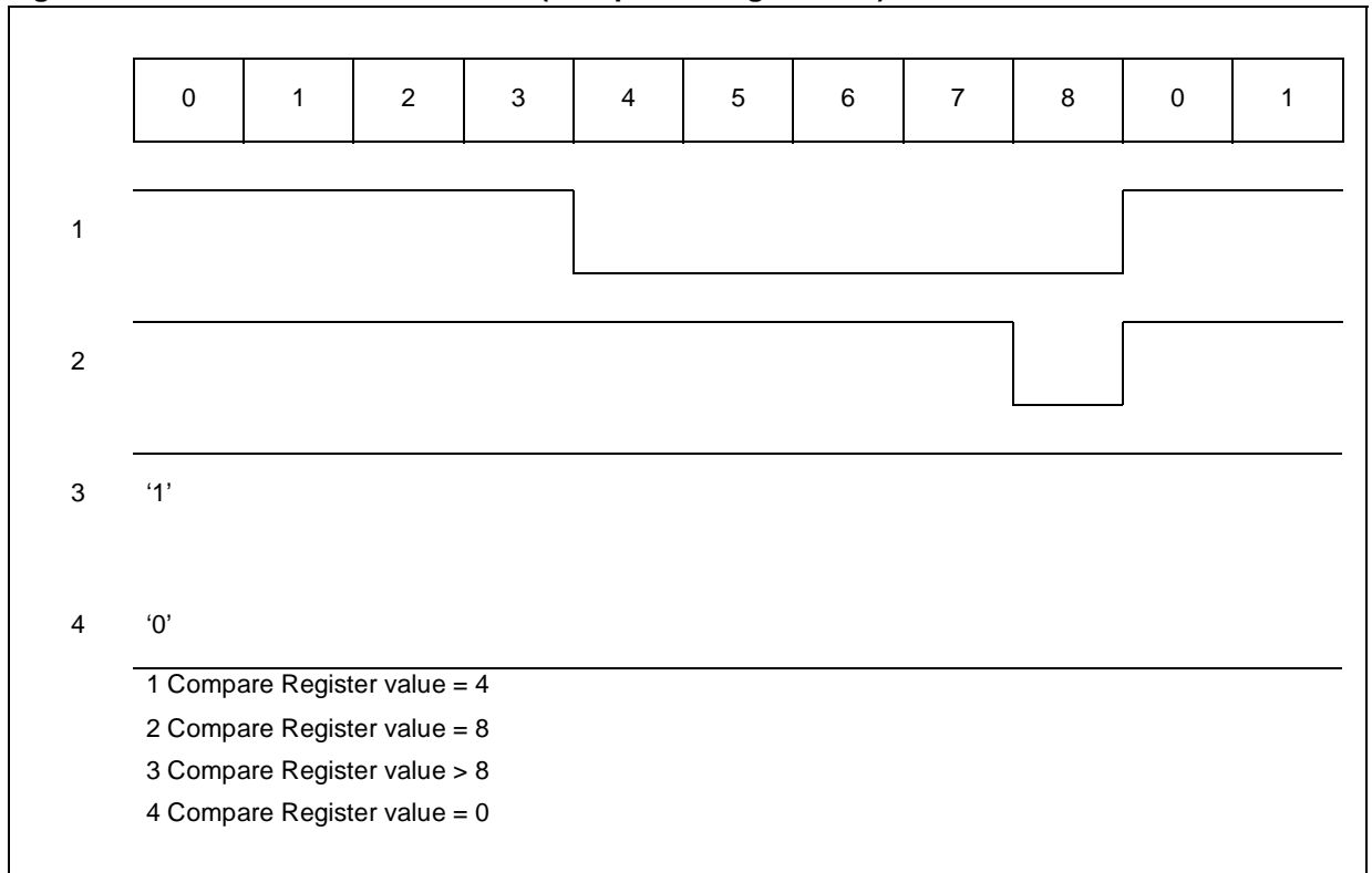
Figure 65. Classical PWM Waveforms (Compare 0 Register = 8)
