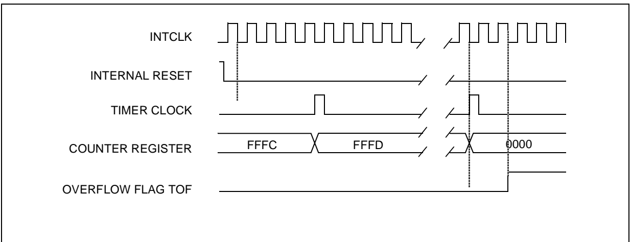
Figure 55. Counter Timing Diagram, INTCLK divided by 8
