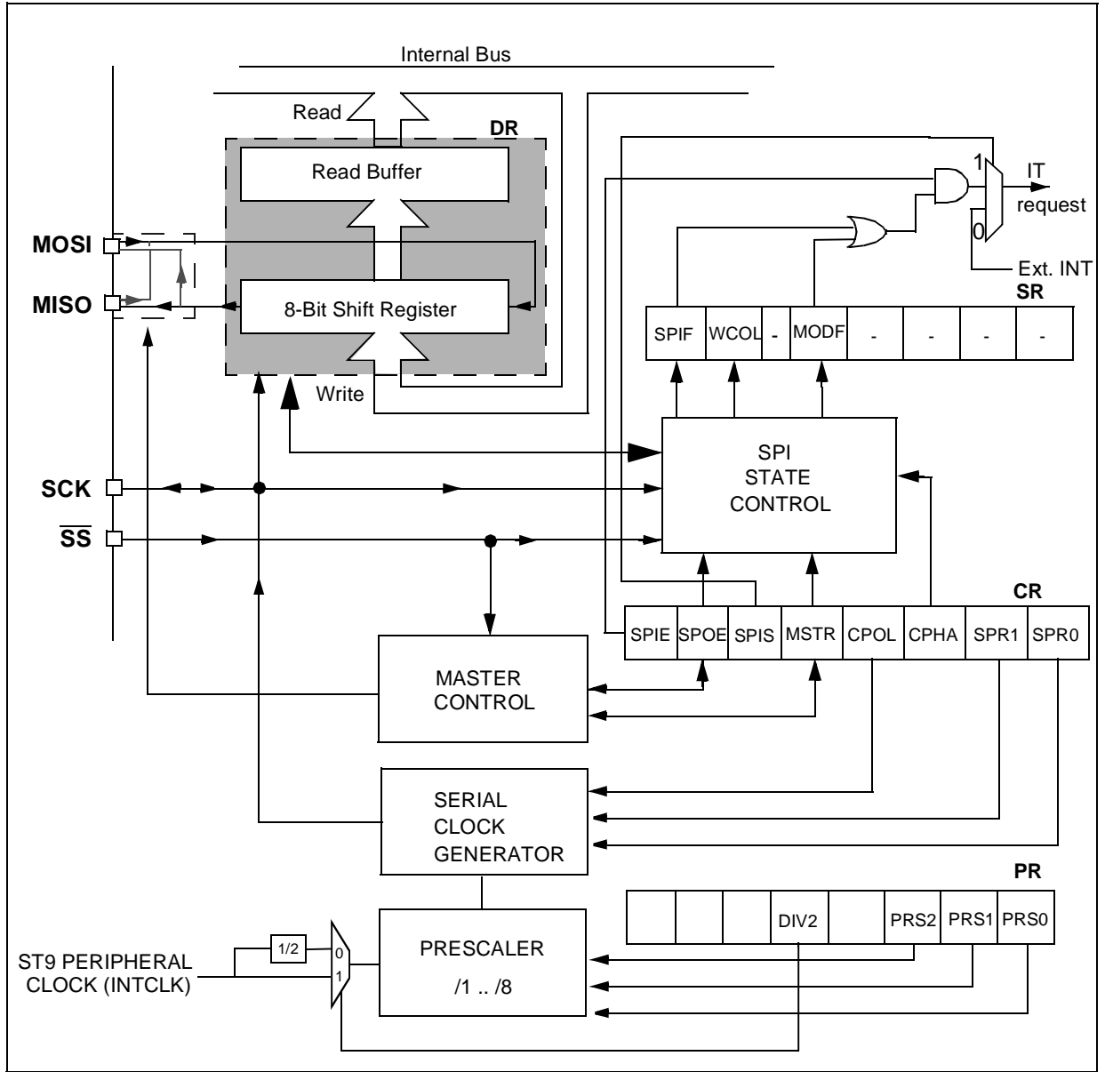
Figure 72. Serial Peripheral Interface Block Diagram
