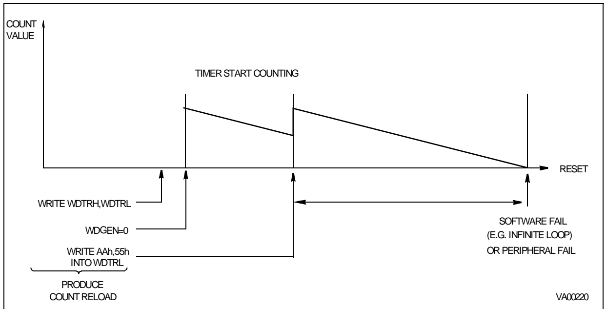
Figure 49. Watchdog Timer Mode
