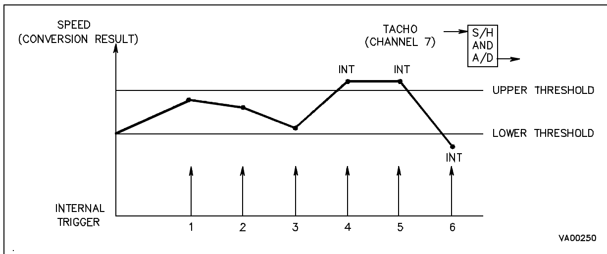
Figure 79. Application Example: Analog Watchdog used in Motorspeed Control
