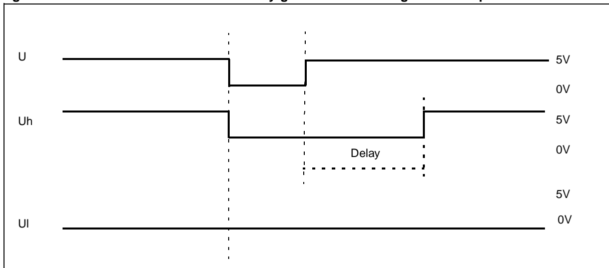
Figure 67. Dead Time waveforms with delay greater than the negative PWM pulse
