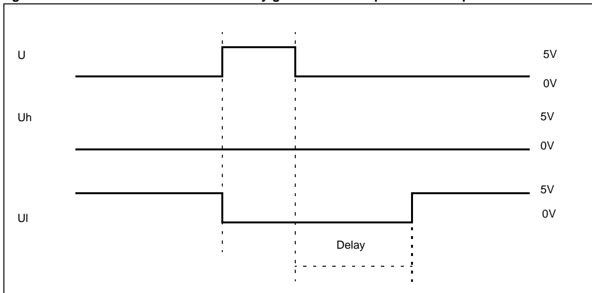
Figure 68. Dead Time waveforms with delay greater than the positive PWM pulse
