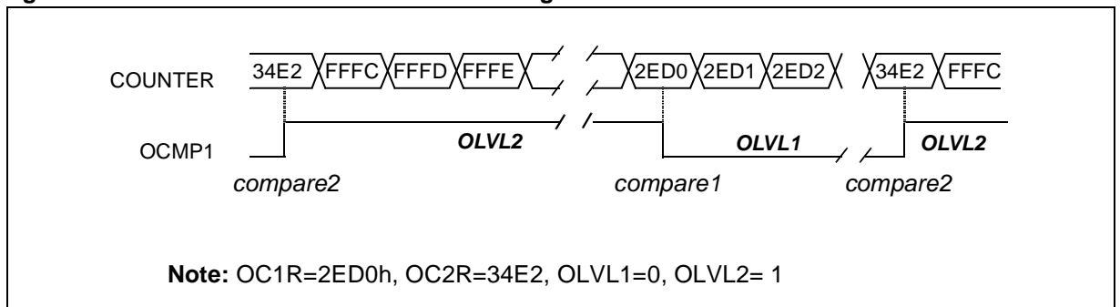
Figure 61. Pulse Width Modulation Mode Timing
