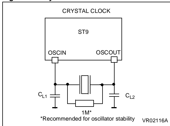
Figure 34. Crystal Oscillator
