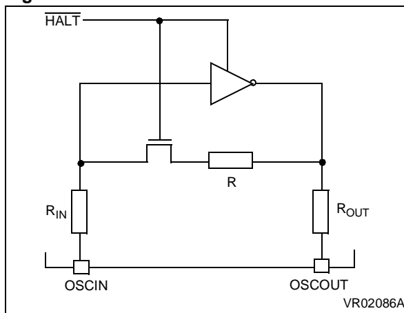
Figure 35. Internal Oscillator Schematic
