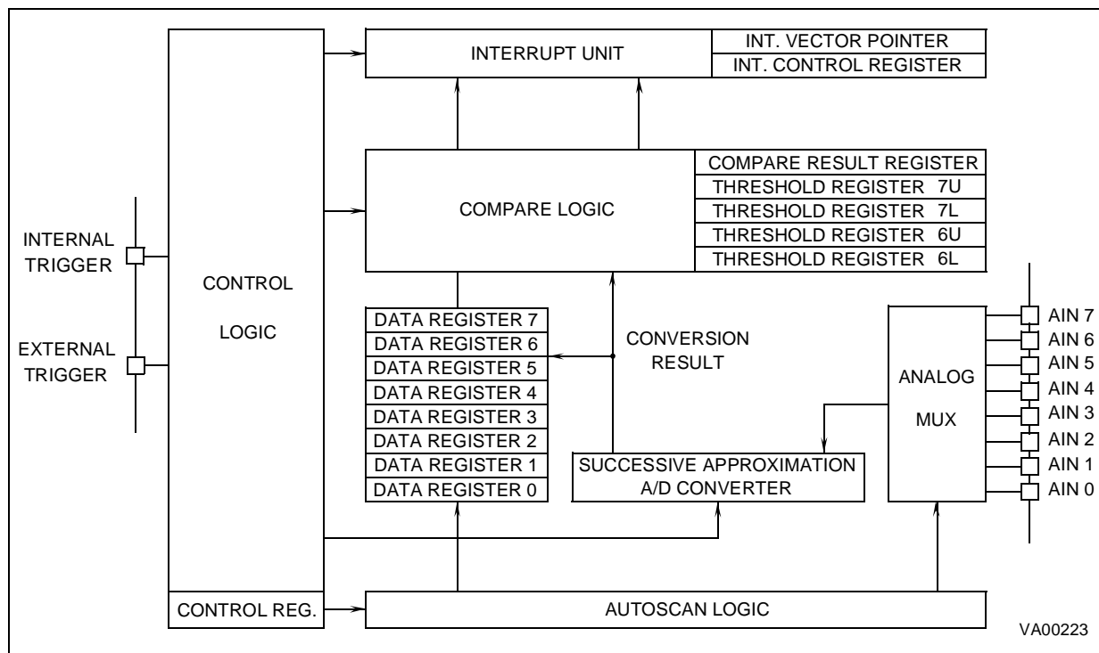
Figure 77. Block Diagram
