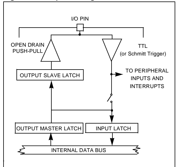
Figure 45. Output Configuration
