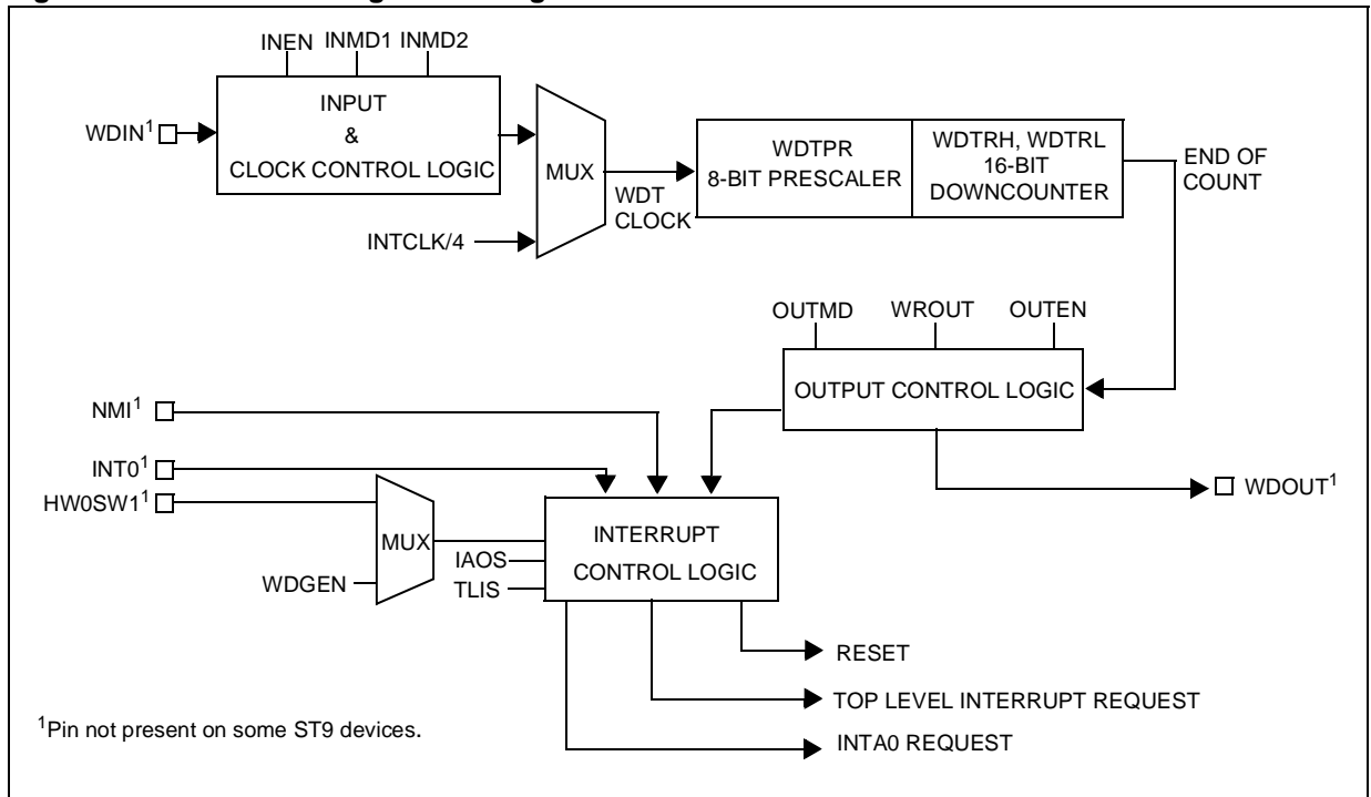
Figure 48. Timer/Watchdog Block Diagram
