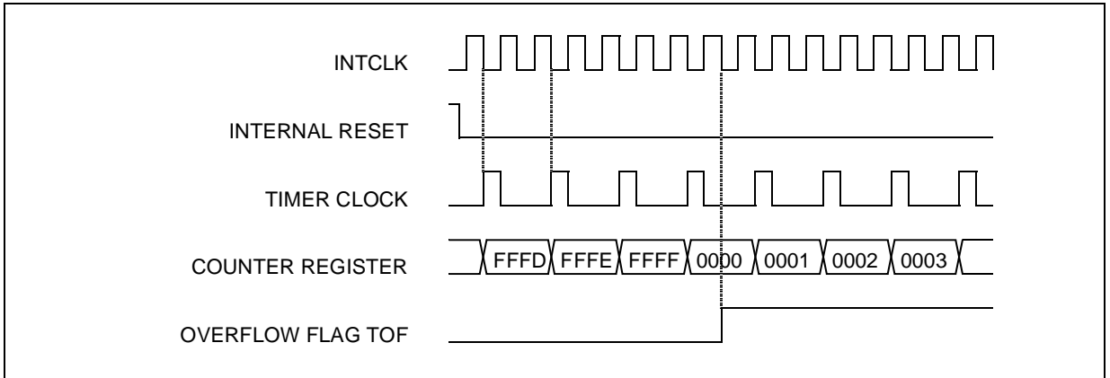
Figure 53. Counter Timing Diagram, INTCLK divided by 2
