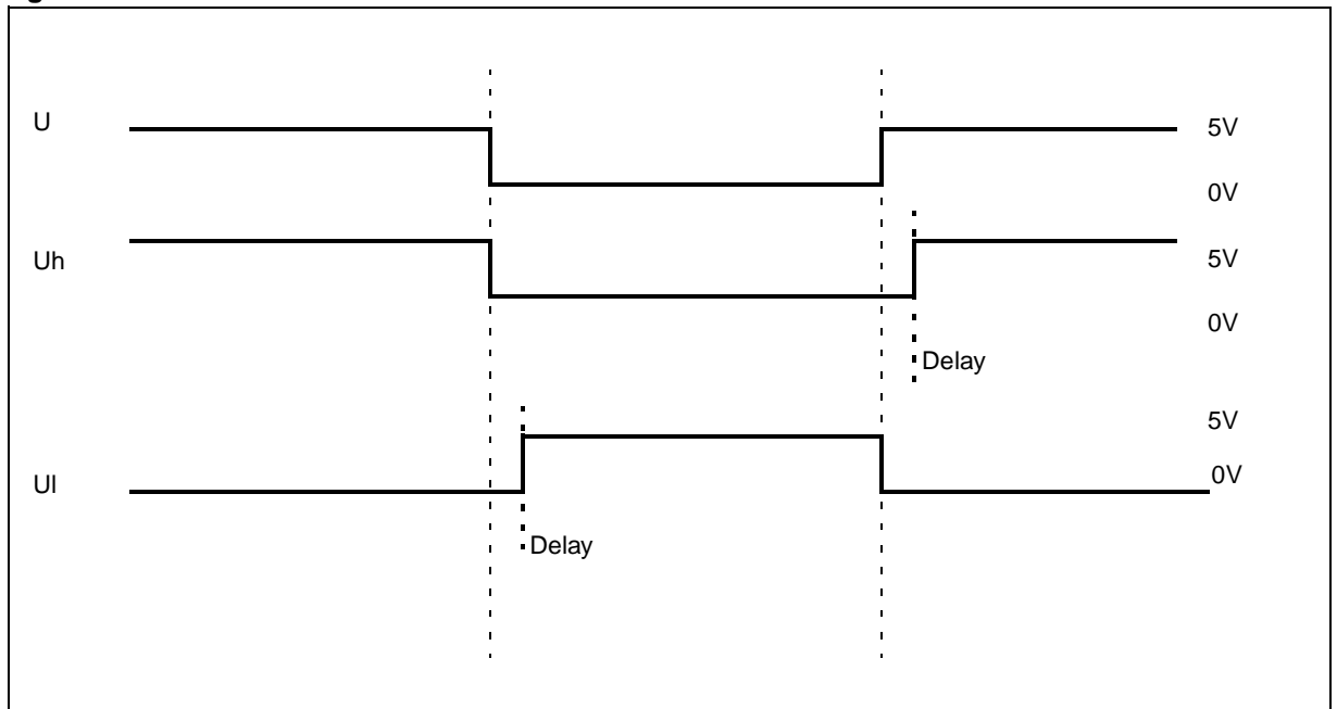
Figure 66. Dead Time waveforms
