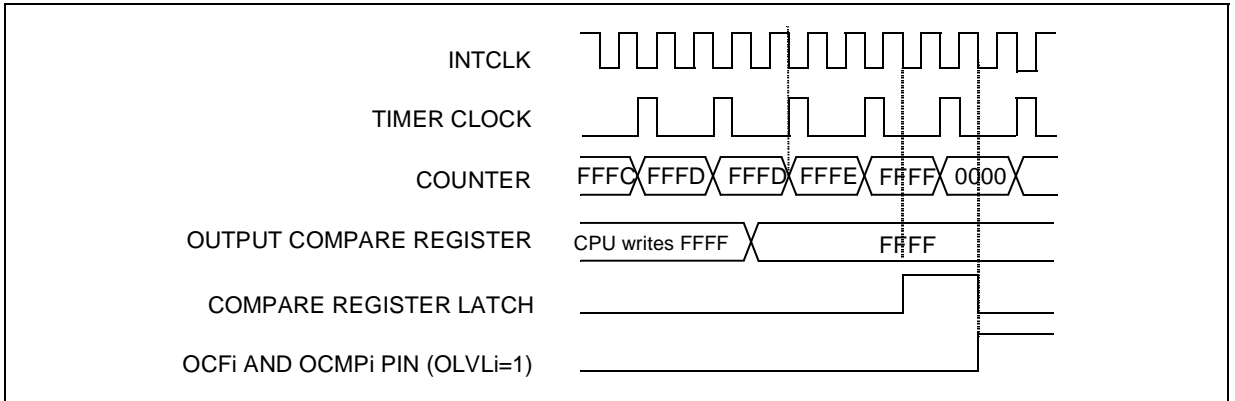
Figure 59. Output Compare Timing Diagram, Internal Clock Divided by 2
