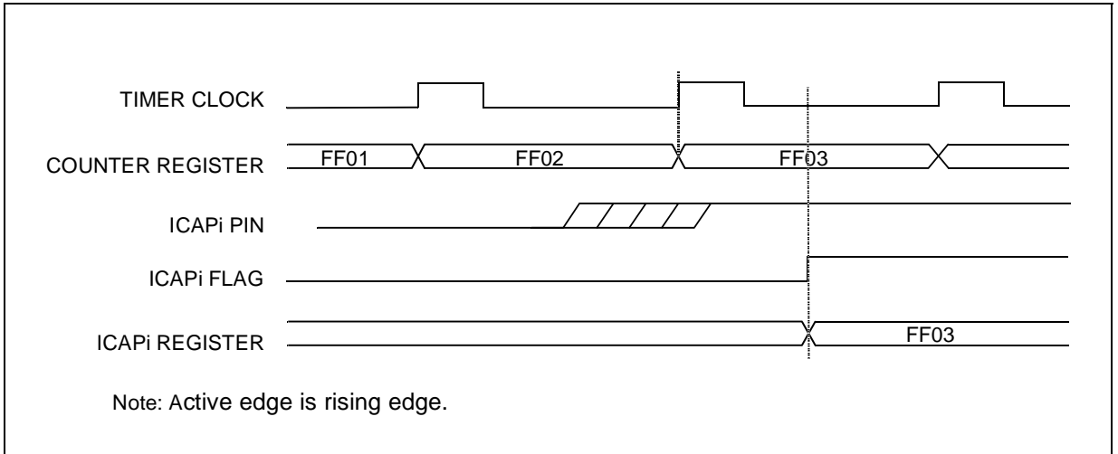
Figure 57. Input Capture Timing Diagram
