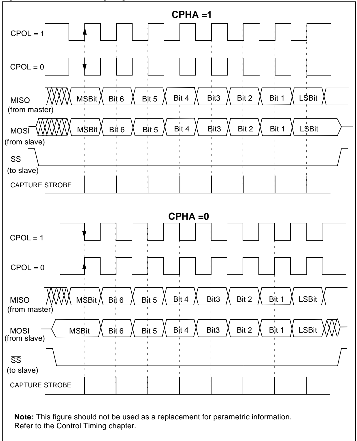
Figure 74. Data Clock Timing Diagram
