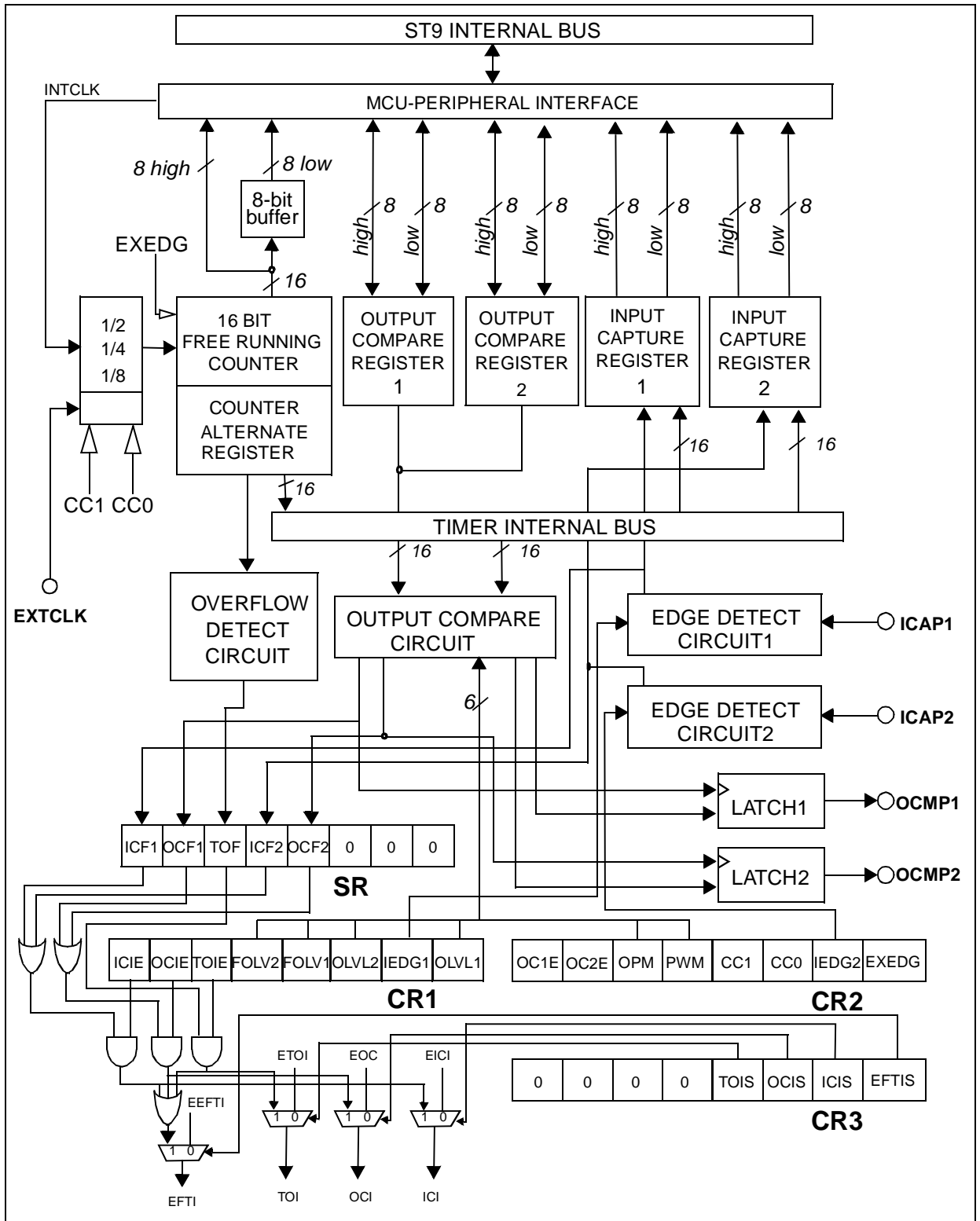
Figure 52. Timer Block Diagram
