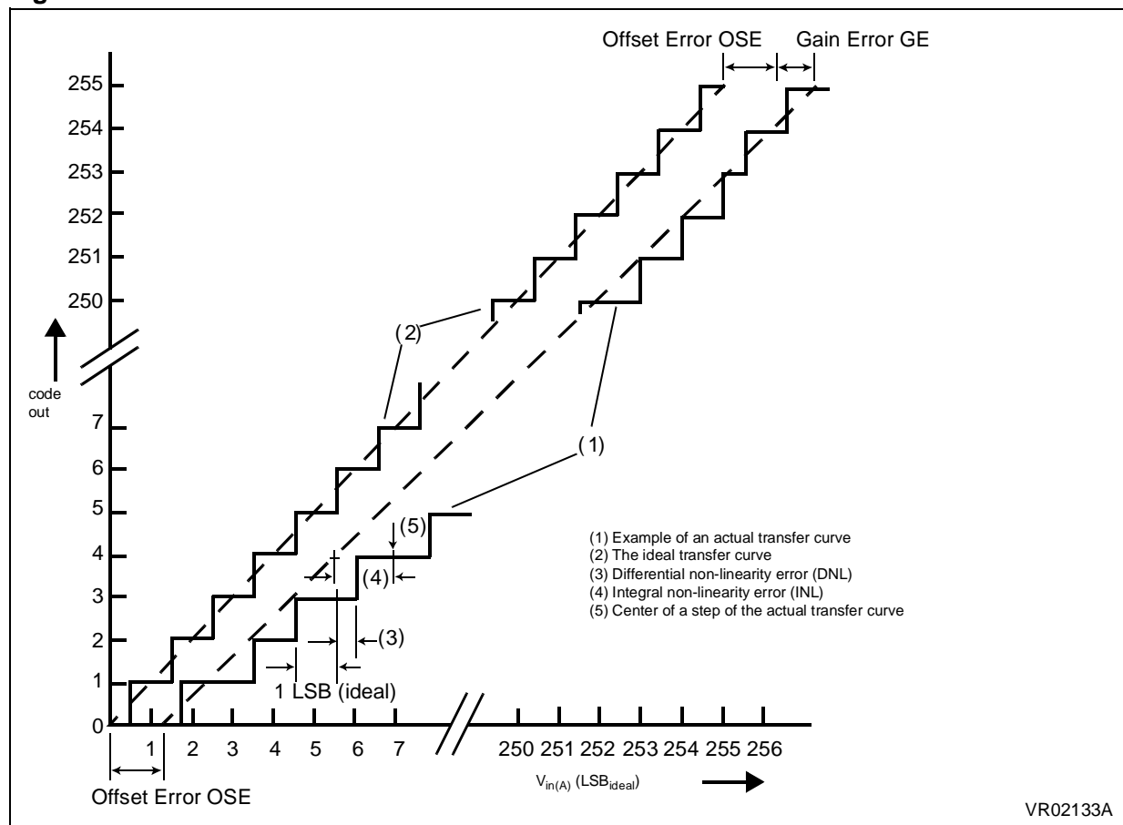
Figure 80. A/D Conversion Characteristics
