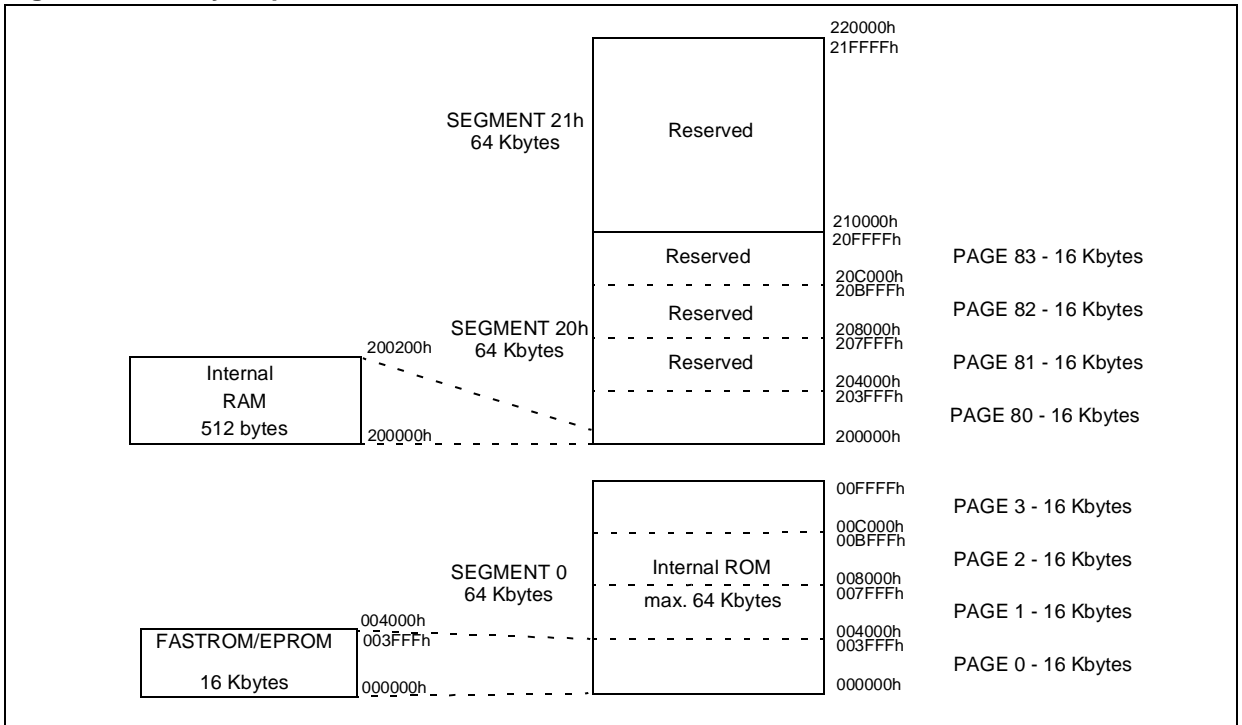
Figure 2. Memory Map
