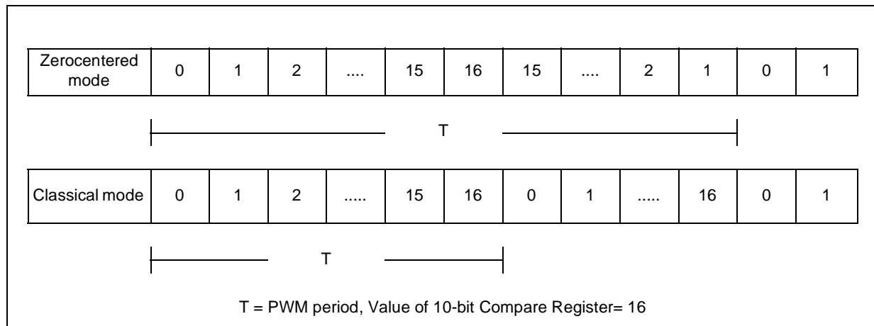
Figure 63. Counting sequence in Zerocentered and Classical mode
