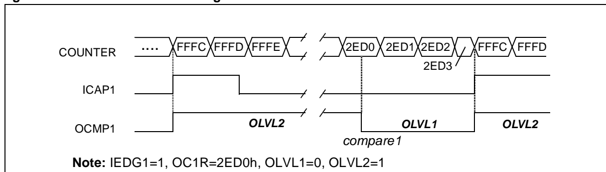
Figure 60. One Pulse Mode Timing
