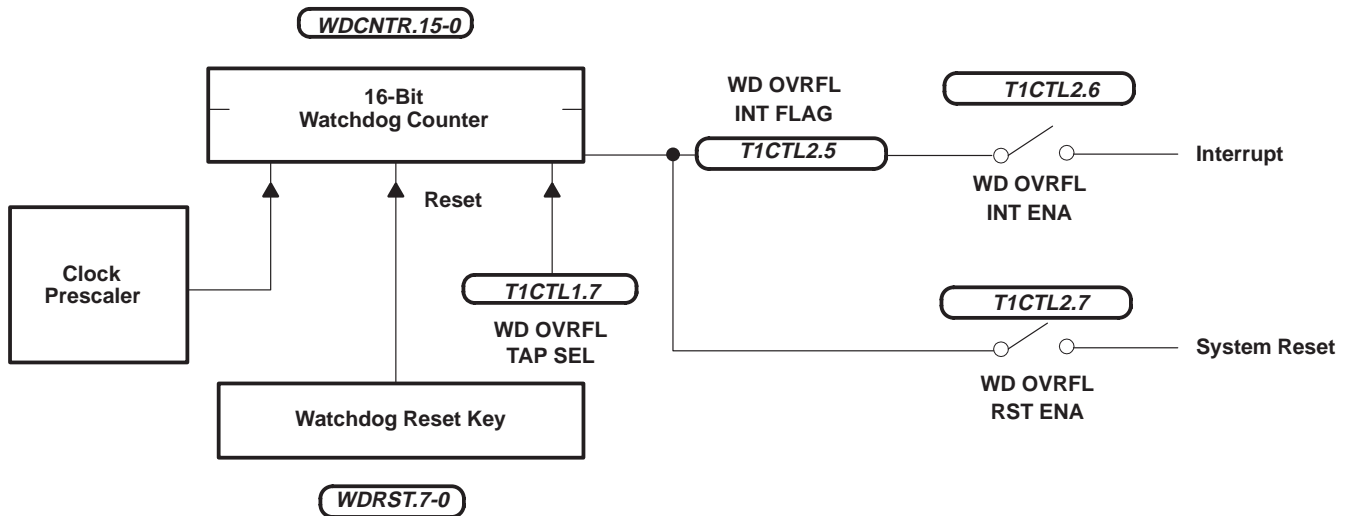
Figure 8. Standard Watchdog
